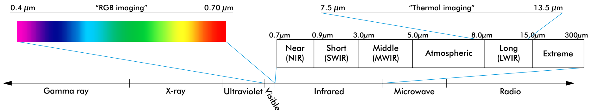
Figure 2: Where daylight cameras and Forward-Looking Infrared Radiometers (FLIRs) operate along the electromagnetic spectrum. Differences in properties of visible light and infrared light lead to differences in camera properties. Daylight cameras and FLIRs are both used for aerial imagery of boreal caribou in Canada. Figure content is based on: NASA 2013, Akhloufi and Bendada 2013, Pinkson 2015, Grainger 2018, FLIR Systems Inc. 2019.
